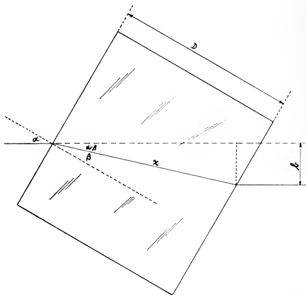
FIG. 1. Plane parallel glass plate penetrated by a light-ray.
